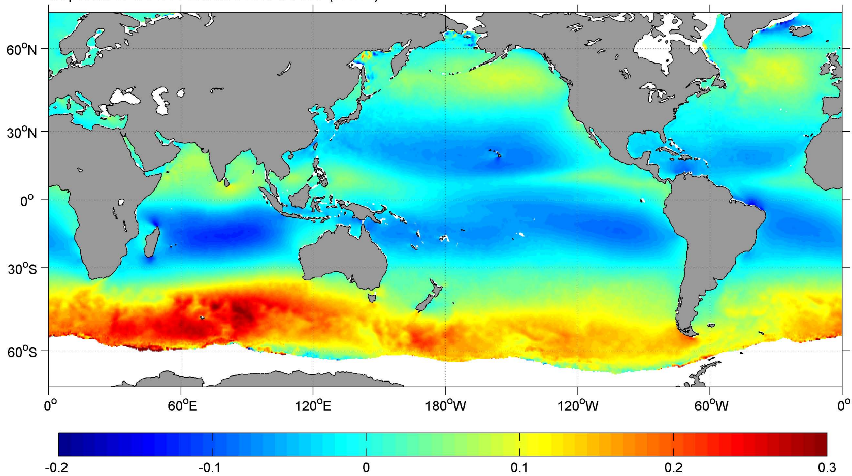
September SCOW Zonal Wind Stress ( \text{N m}^{-2} )
