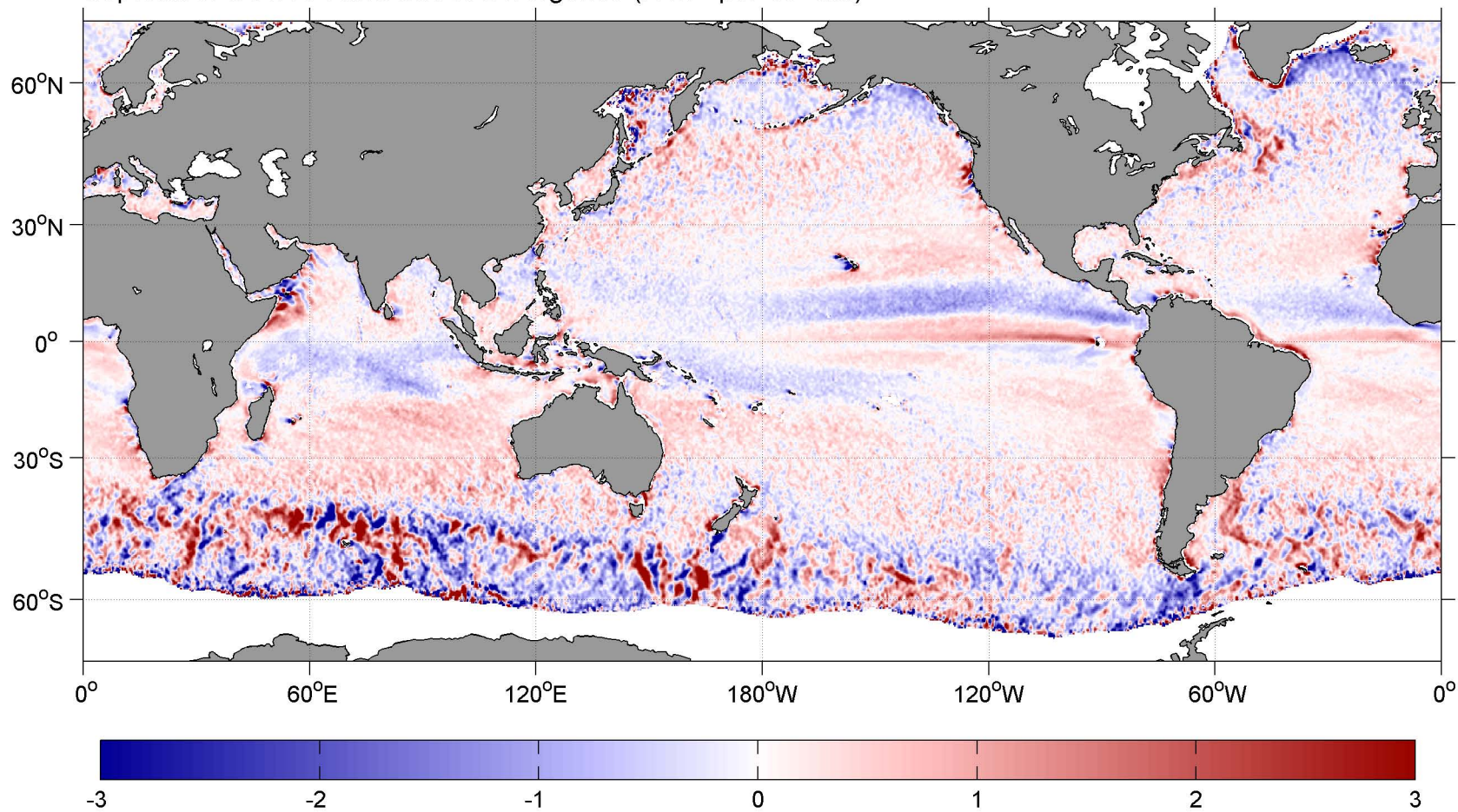
September SCOW Wind Stress Divergence ( \text{N m}^{-2} per 10^4 \text{ km}^2 )
