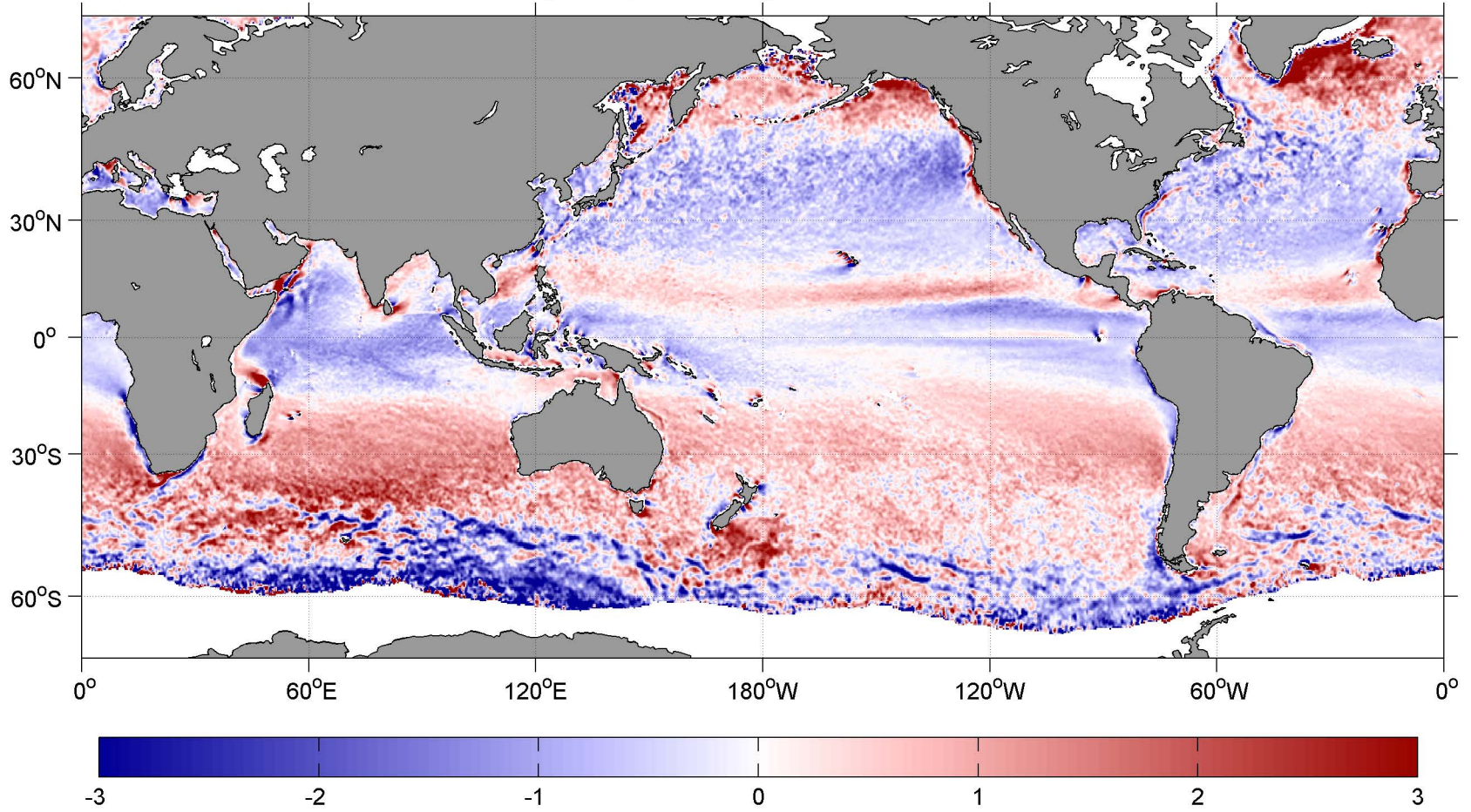
September SCOW Wind Stress Curl ( \text{N m}^{-2} per 10^4 \text{ km} )
