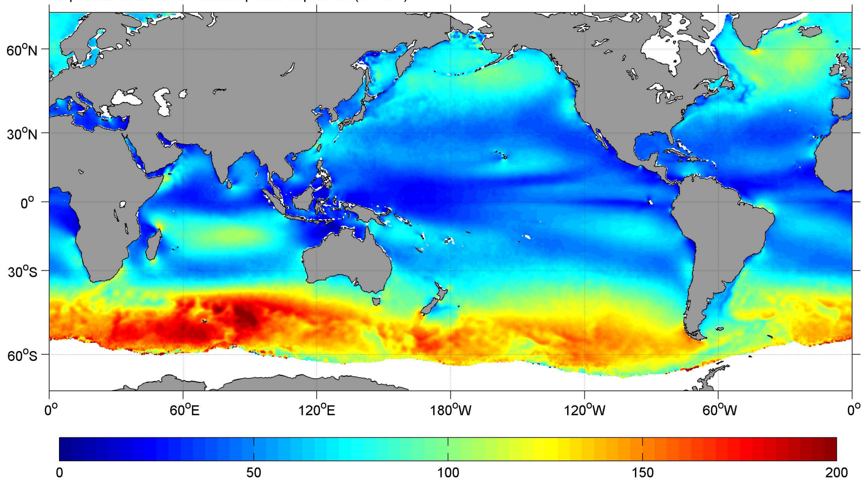
September SCOW Wind Speed Squared ( \text{m}^2 \text{s}^{-2} )
