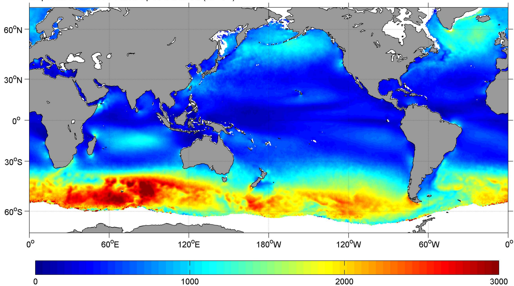
September SCOW Wind Speed Cubed ( \text{m}^3 \text{s}^{-3} )
