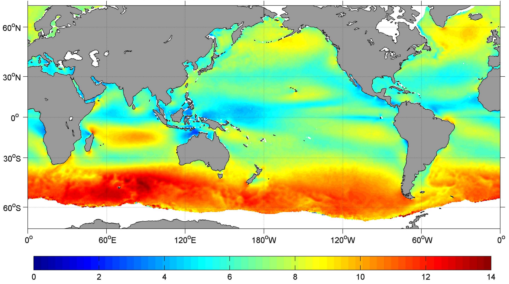
September SCOW Wind Speed ( \text{m s}^{-1} )
