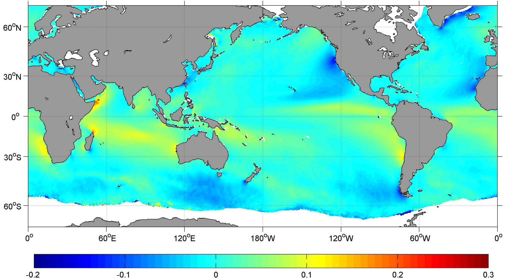
September SCOW Meridional Wind Stress ( \text{N m}^{-2} )
