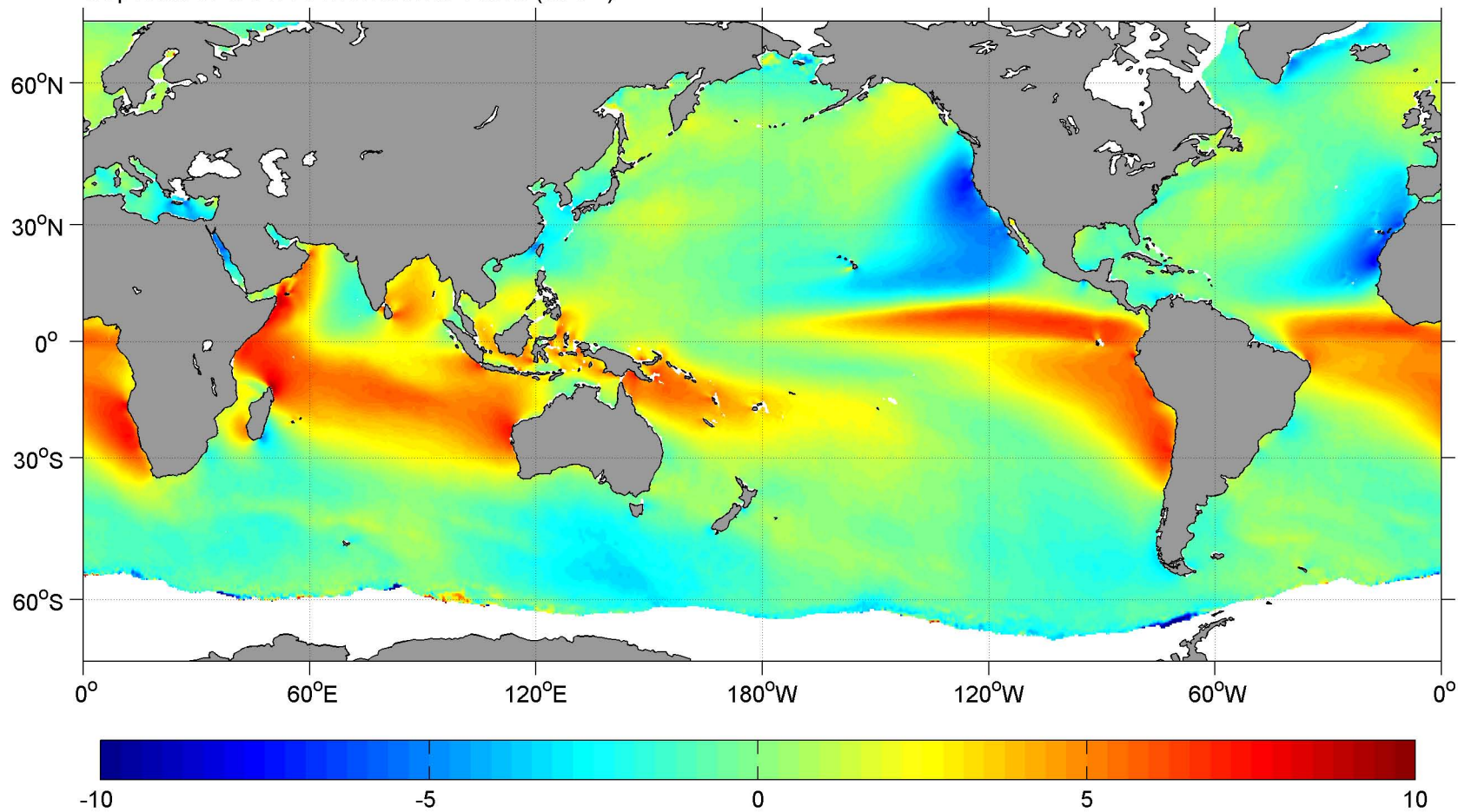
September SCOW Meridional Wind ( \text{m s}^{-1} )
