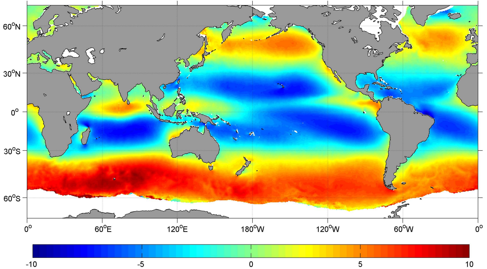
October SCOW Zonal Wind ( \text{m s}^{-1} )
