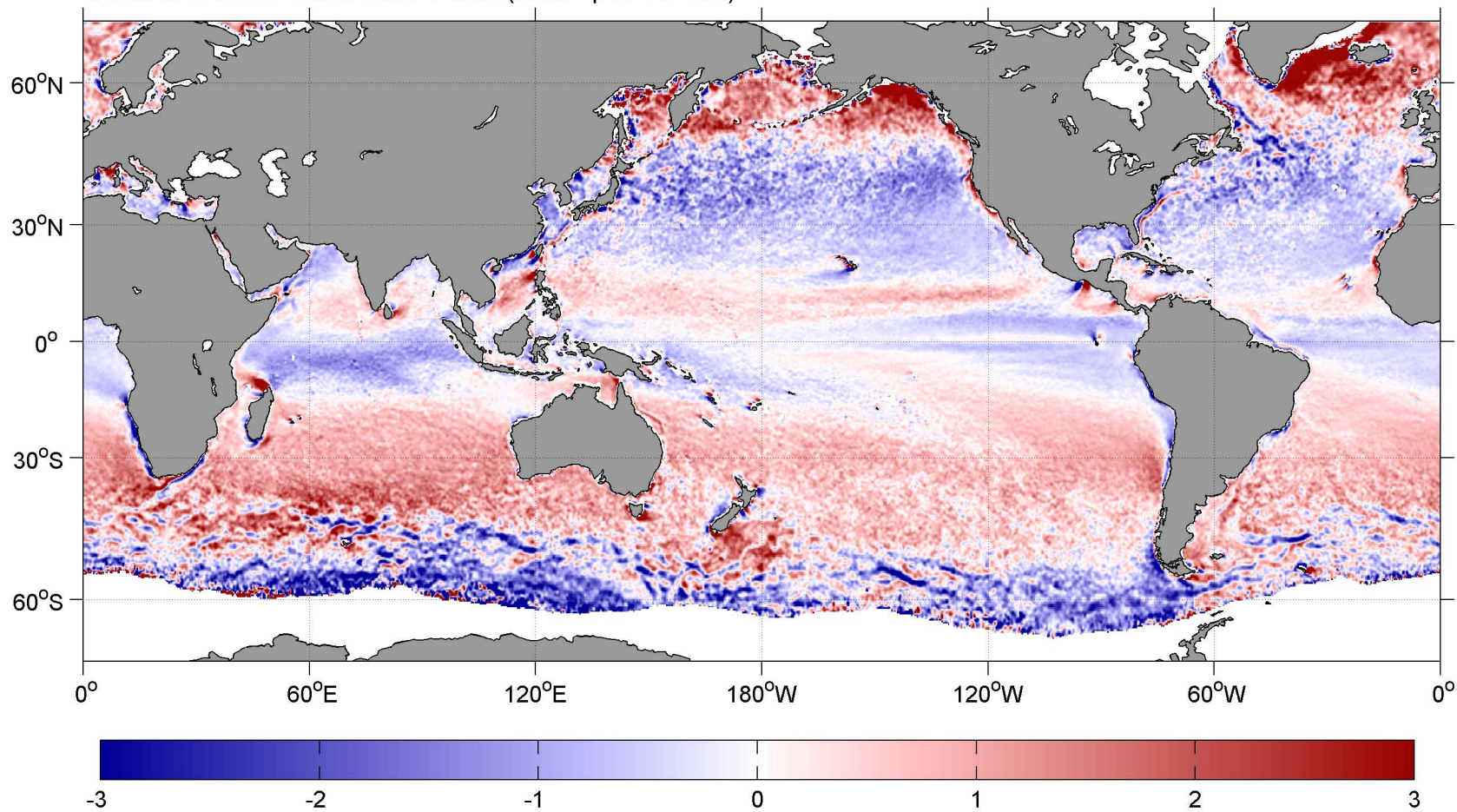
October SCOW Wind Stress Curl ( \text{N m}^{-2} per 10^4 \text{ km}^2 )
