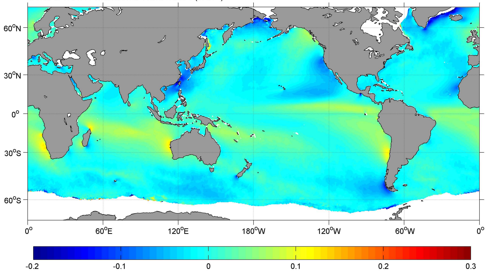
October SCOW Meridional Wind Stress ( \text{N m}^{-2} )
