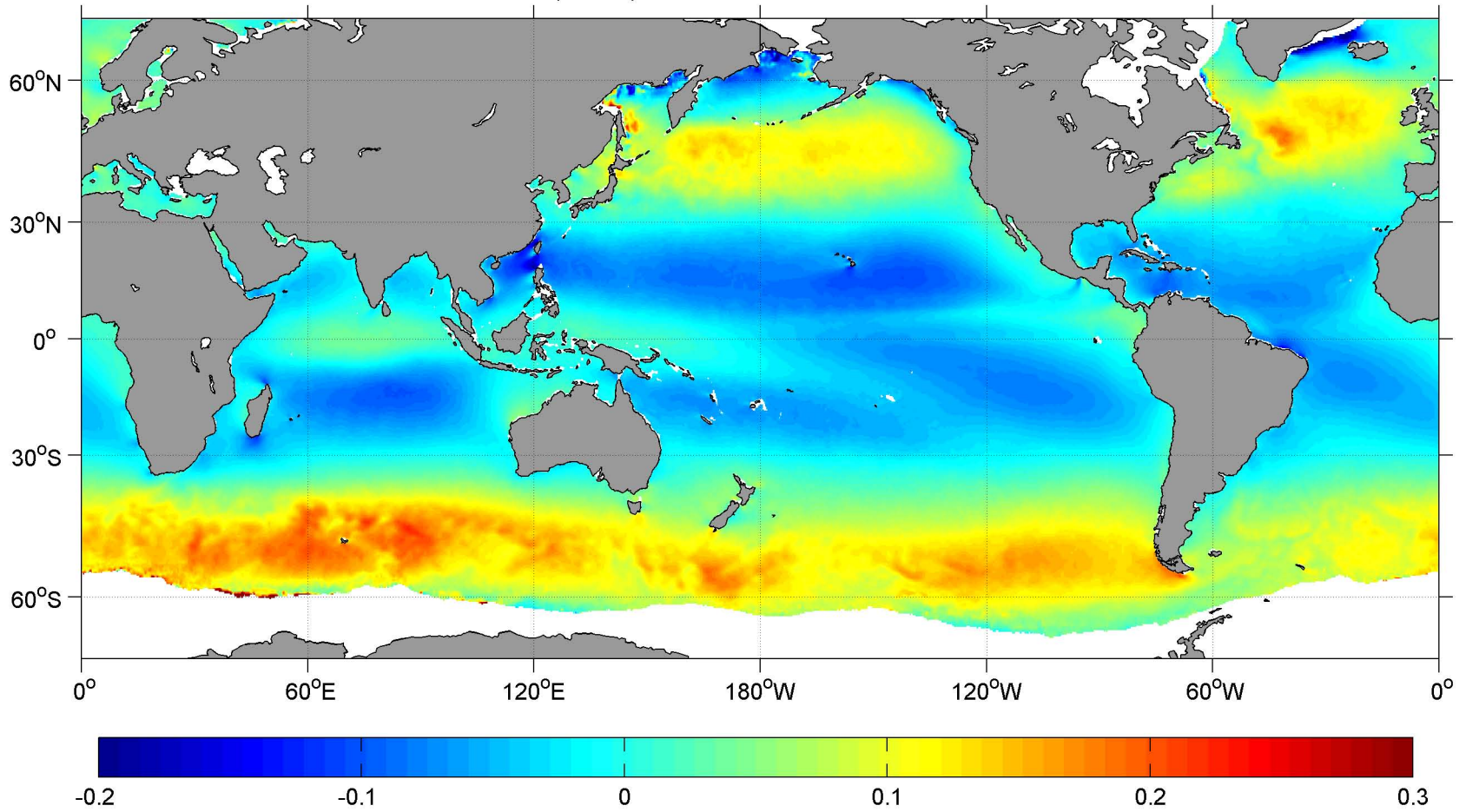
November SCOW Zonal Wind Stress ( \text{N m}^{-2} )
