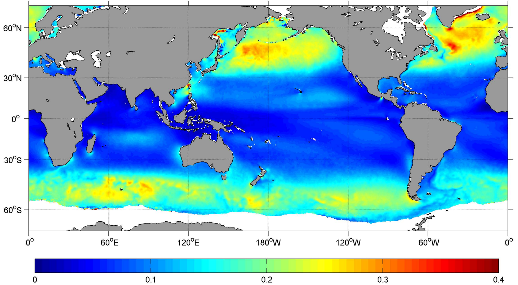
November SCOW Wind Stress Magnitude ( \text{N m}^{-2} )
