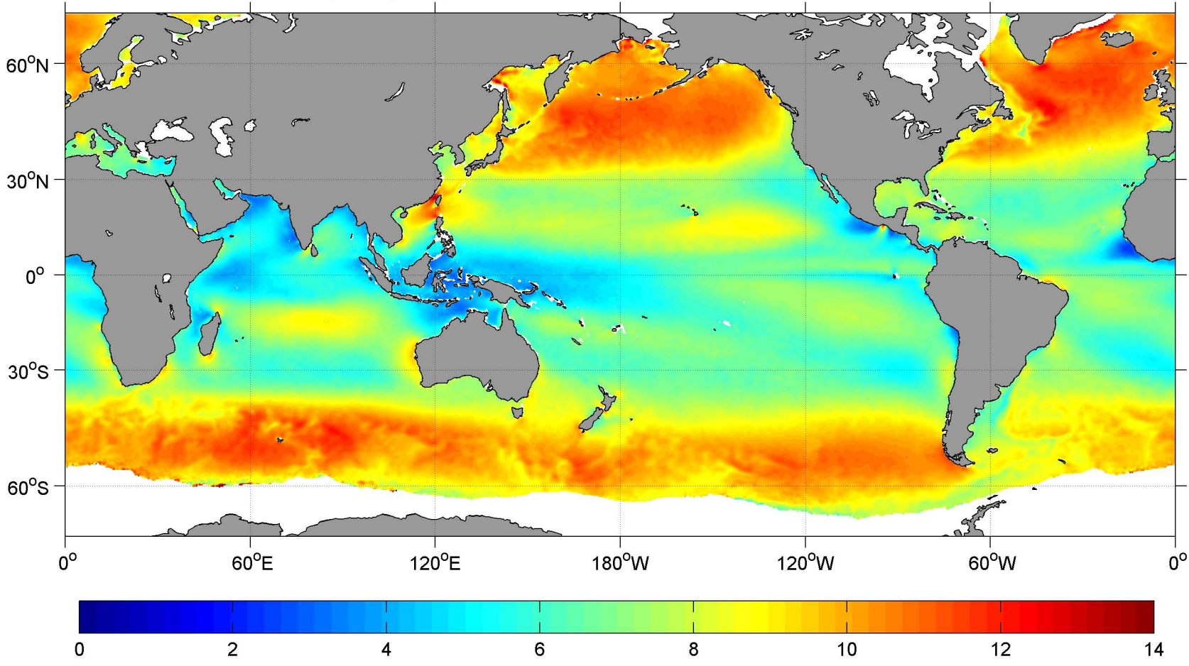
November SCOW Wind Speed ( \text{m s}^{-1} )
