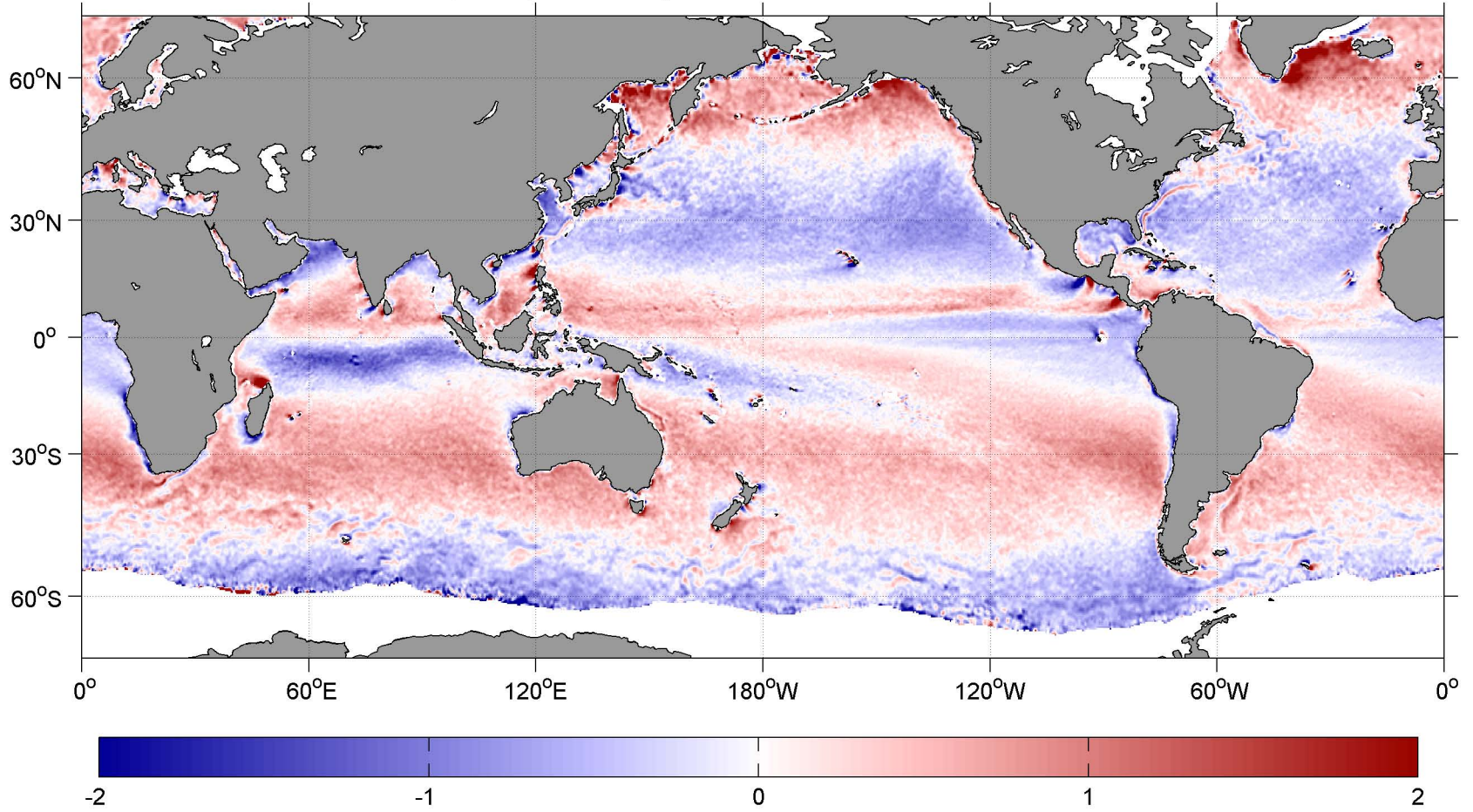
November SCOW Wind Curl ( \text{m s}^{-1} per 10^2 \text{ km} )
