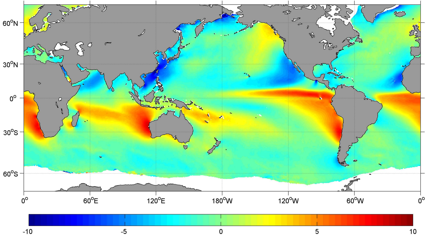
November SCOW Meridional Wind ( \text{m s}^{-1} )
