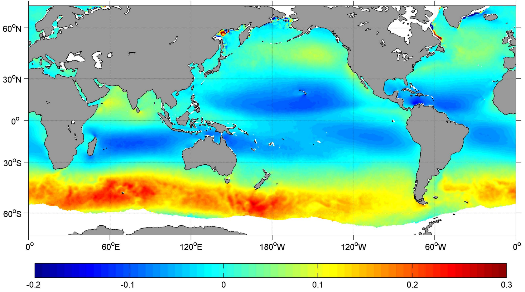
May SCOW Zonal Wind Stress ( \text{N m}^{-2} )
