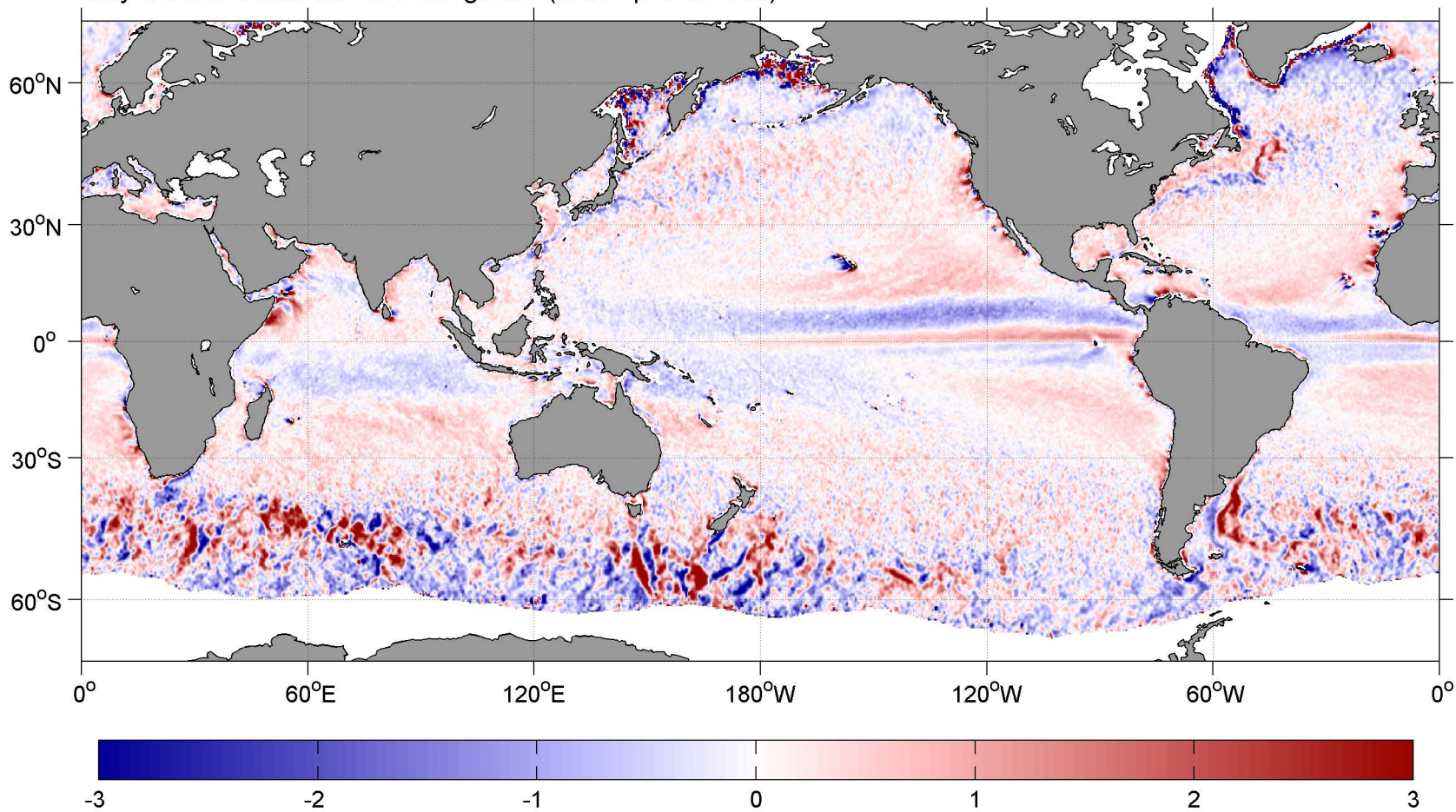
May SCOW Wind Stress Divergence ( \text{N m}^{-2} per 10^4 \text{ km}^2 )
