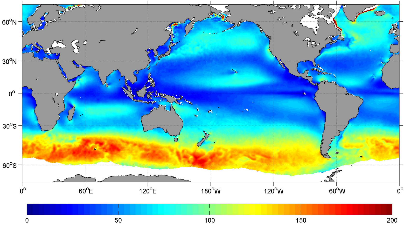
May SCOW Wind Speed Squared ( \text{m}^2 \text{s}^{-2} )
