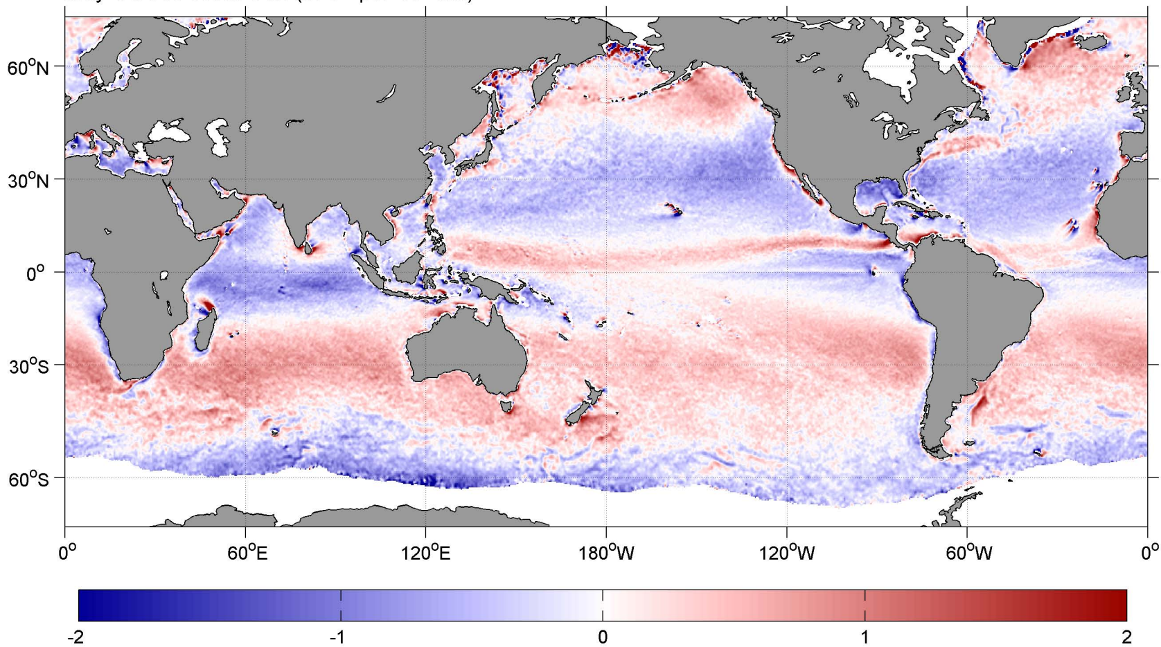
May SCOW Wind Curl ( \text{m s}^{-1} per 10^2 \text{ km} )
