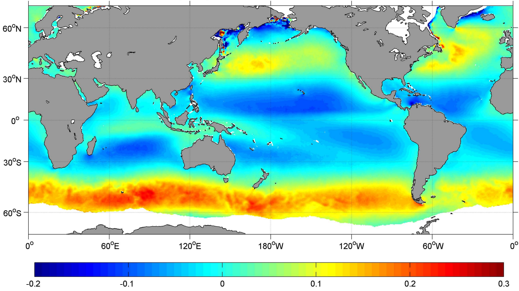
March SCOW Zonal Wind Stress ( \text{N m}^{-2} )
