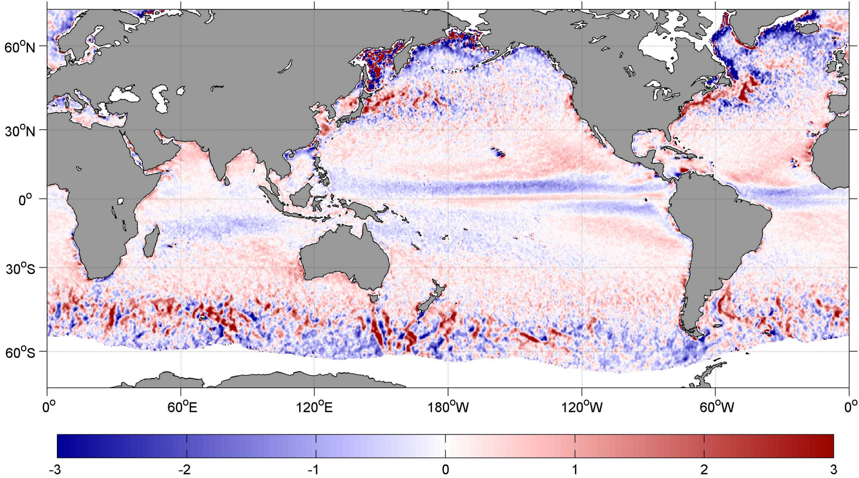
March SCOW Wind Stress Divergence ( \text{N m}^{-2} per 10^4 \text{ km}^2 )
