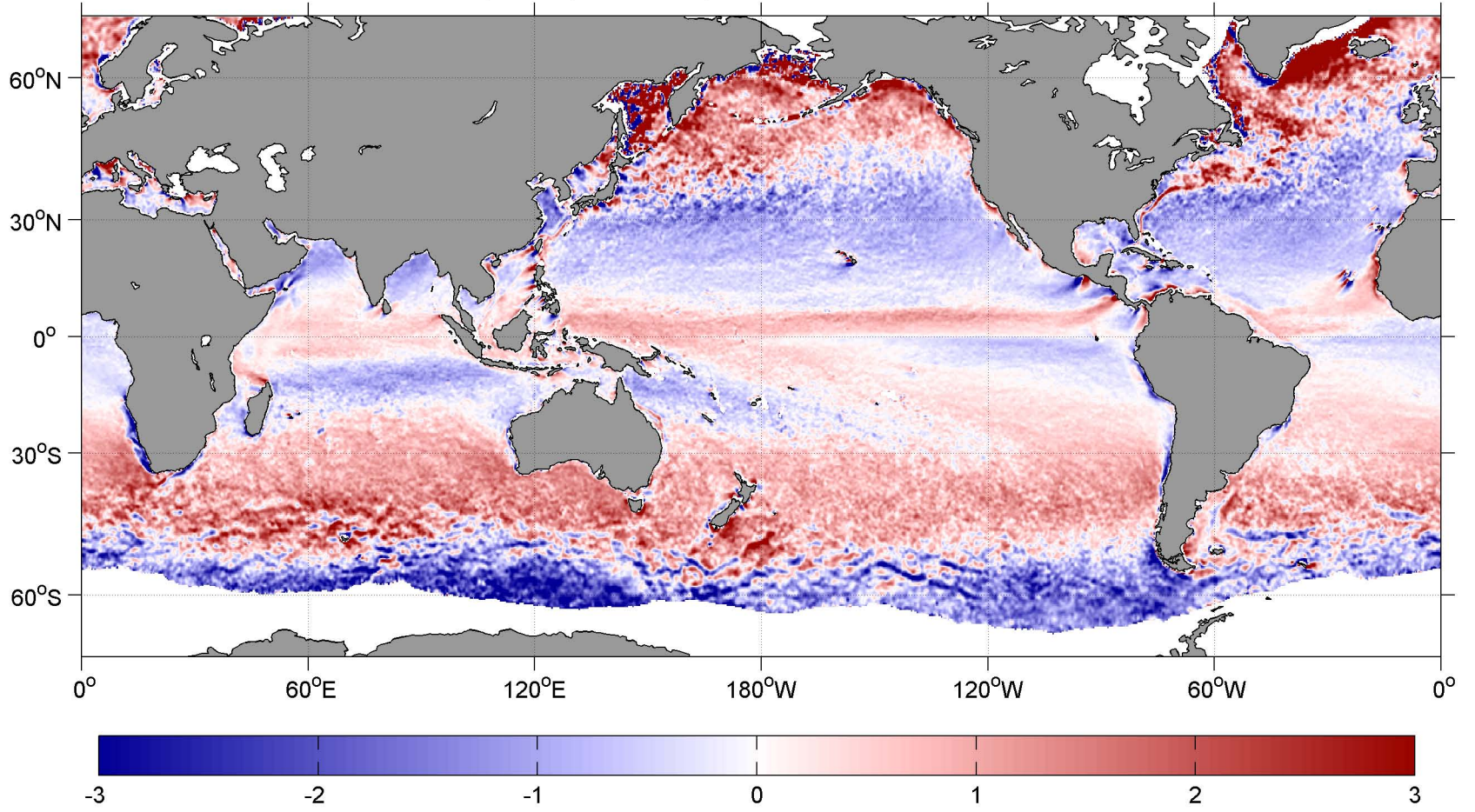
March SCOW Wind Stress Curl ( \text{N m}^{-2} per 10^4 \text{ km}^2 )
