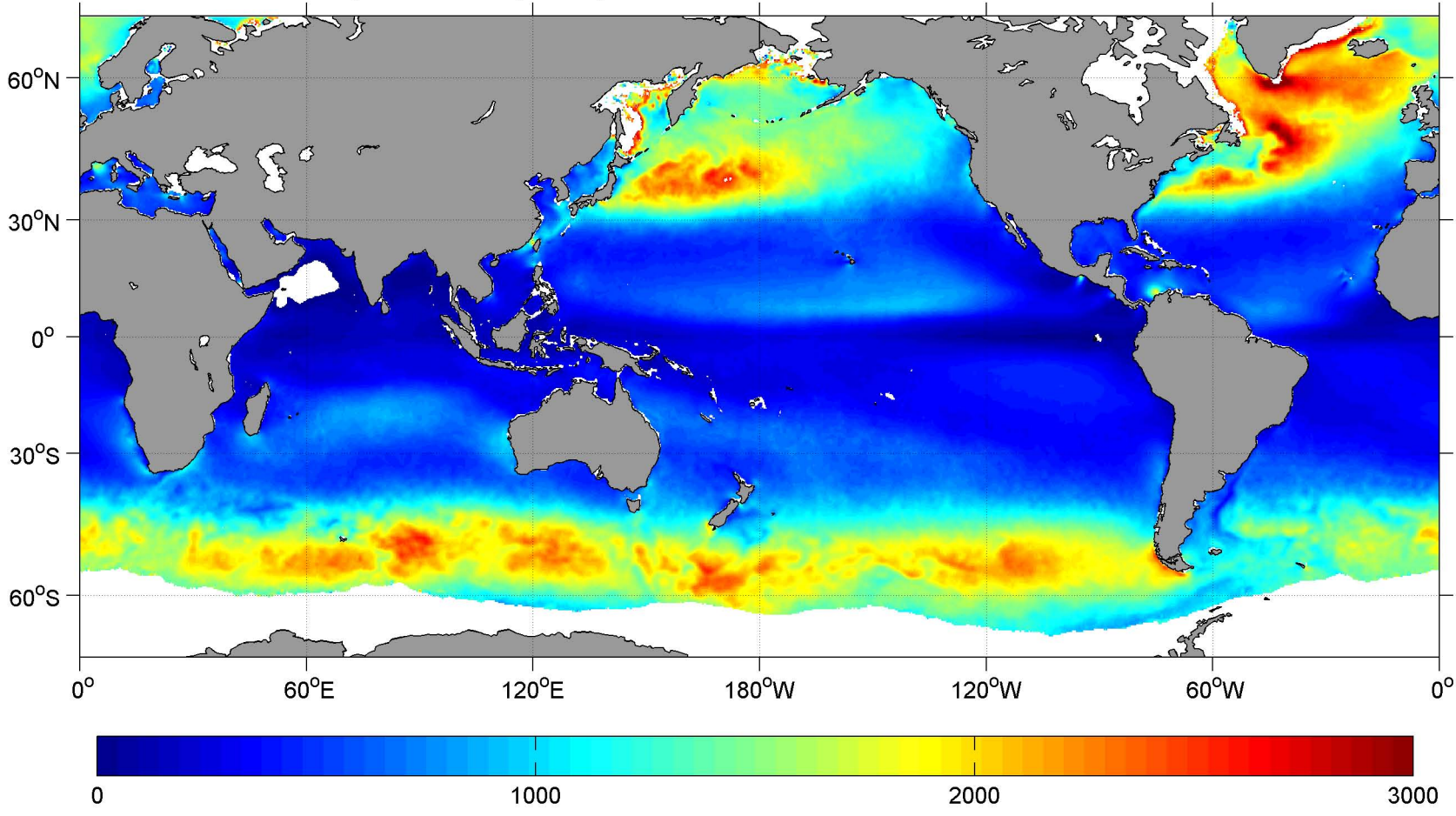
March SCOW Wind Speed Cubed ( \text{m}^3 \text{s}^{-3} )
