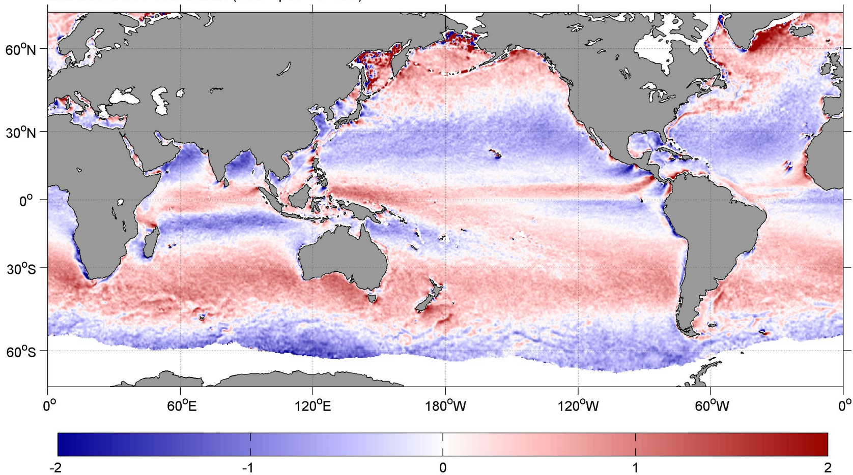
March SCOW Wind Curl ( \text{m s}^{-1} per 10^2 \text{ km} )
