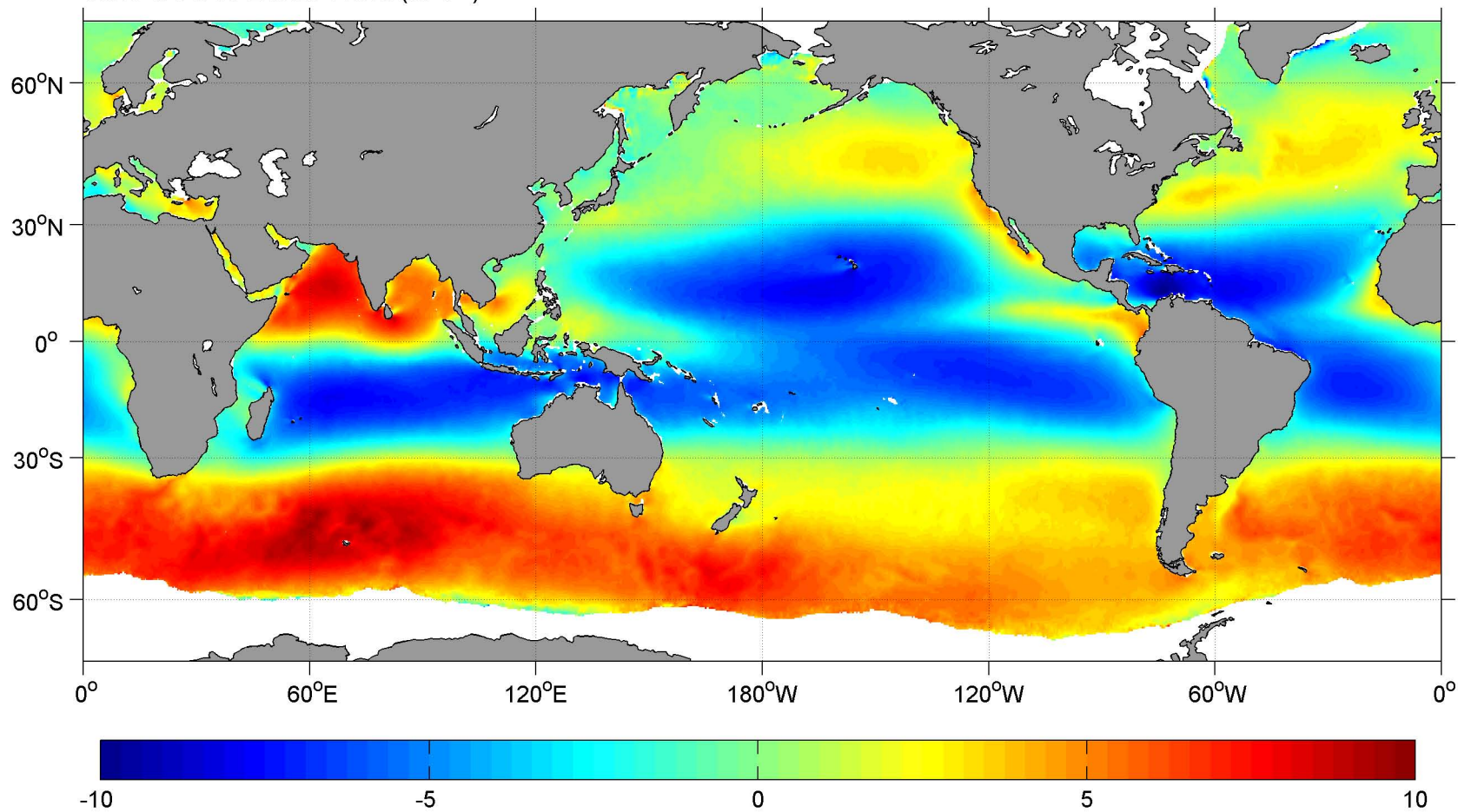
June SCOW Zonal Wind ( \text{m s}^{-1} )
