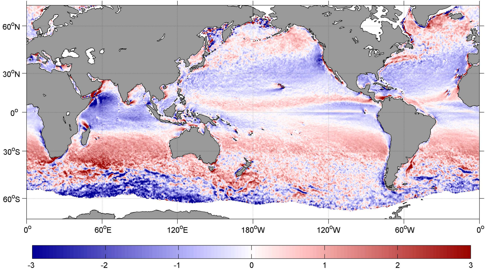
June SCOW Wind Stress Curl ( \text{N m}^{-2} per 10^4 \text{ km} )
