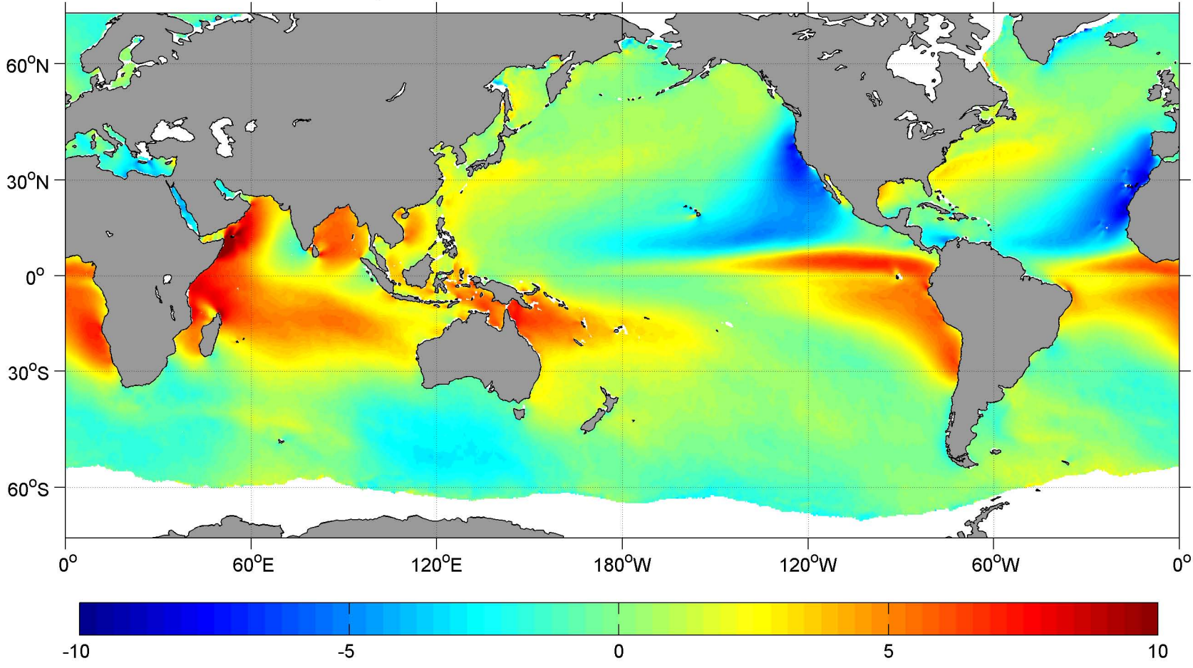
June SCOW Meridional Wind ( \text{m s}^{-1} )
