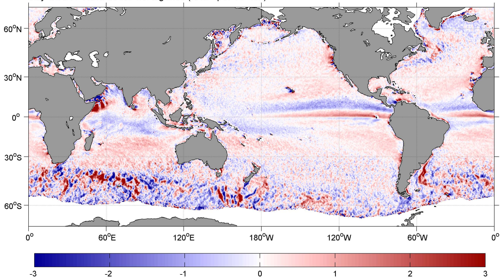
July SCOW Wind Stress Divergence ( \text{N m}^{-2} per 10^4 \text{ km}^2 )
