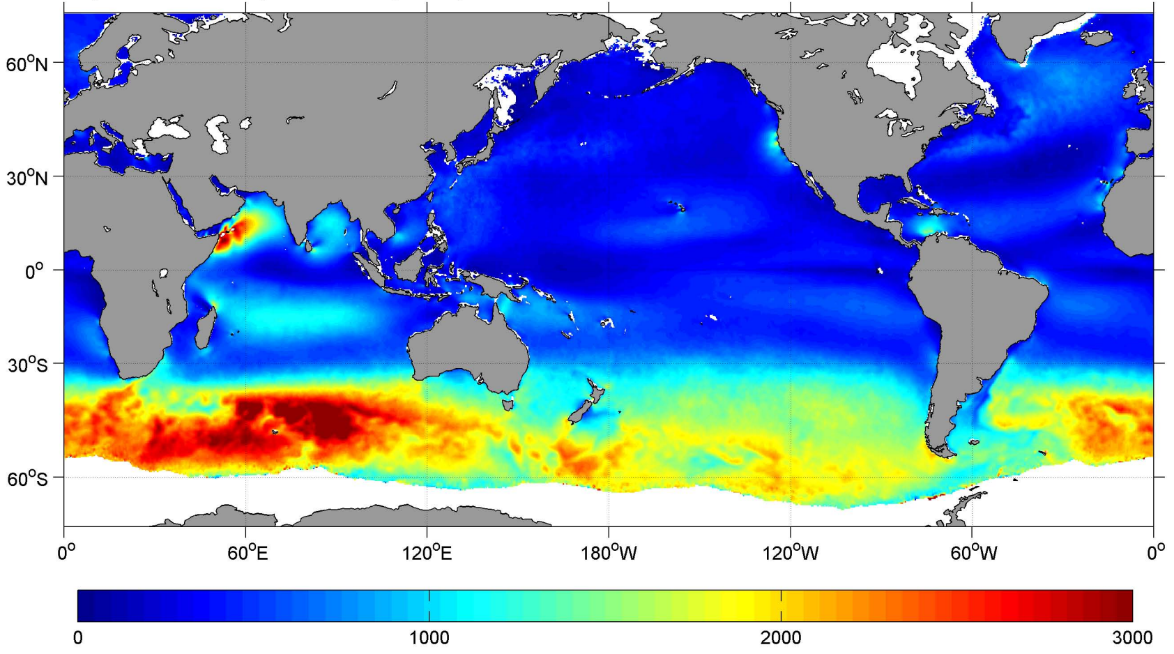
July SCOW Wind Speed Cubed ( \text{m}^3 \text{s}^{-3} )
