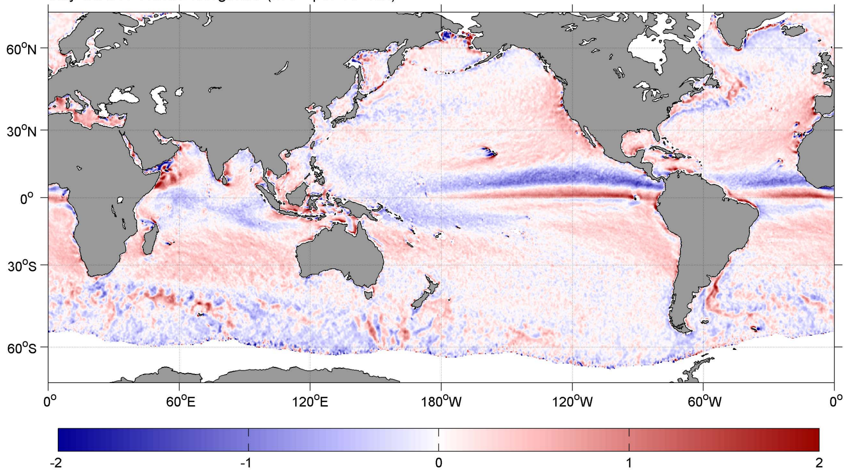
July SCOW Wind Divergence ( \text{m s}^{-1} per 10^2 \text{ km} )
