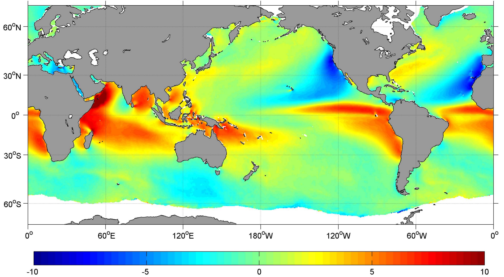
July SCOW Meridional Wind ( \text{m s}^{-1} )
