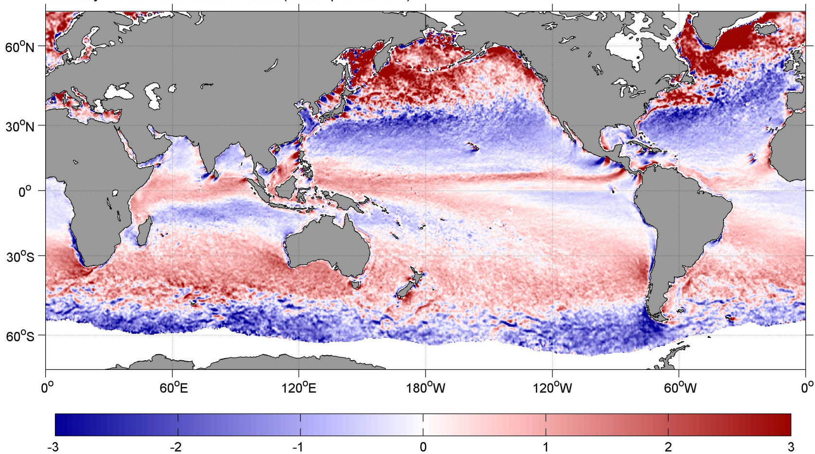
January SCOW Wind Stress Curl ( \text{N m}^{-2} per 10^4 \text{ km}^2 )
