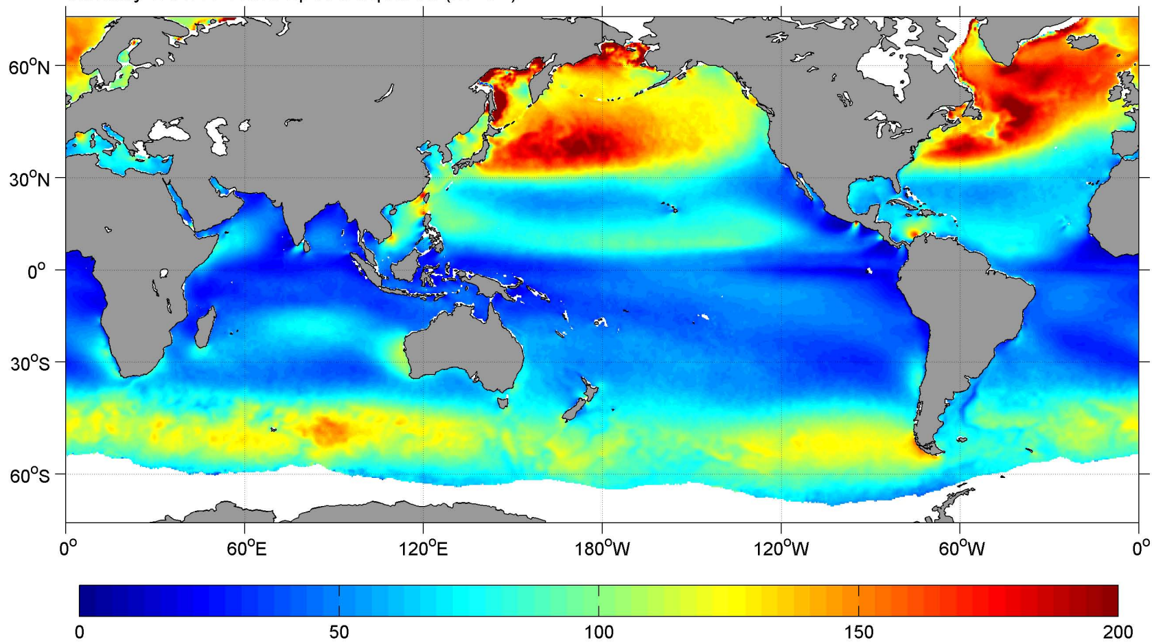
January SCOW Wind Speed Squared ( \text{m}^2 \text{s}^{-2} )
