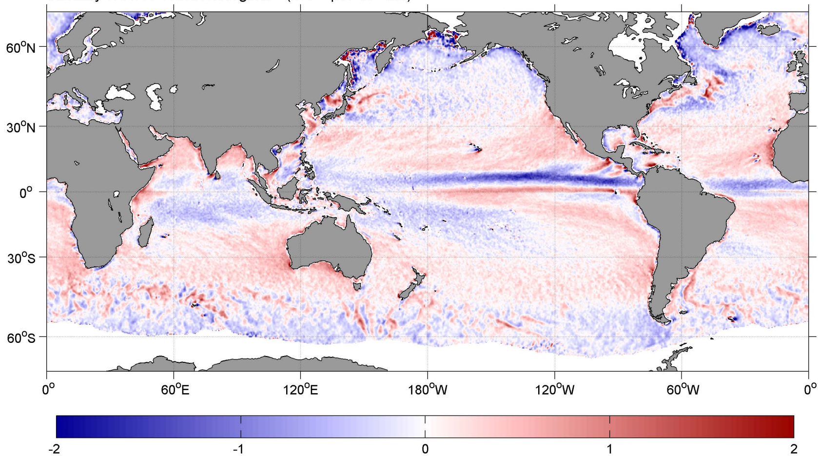
January SCOW Wind Divergence ( \text{m s}^{-1} per 10^2 \text{ km} )
