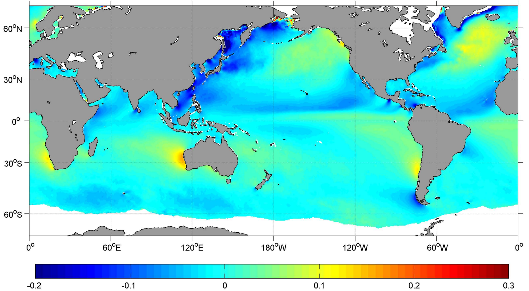
January SCOW Meridional Wind Stress ( \text{N m}^{-2} )
