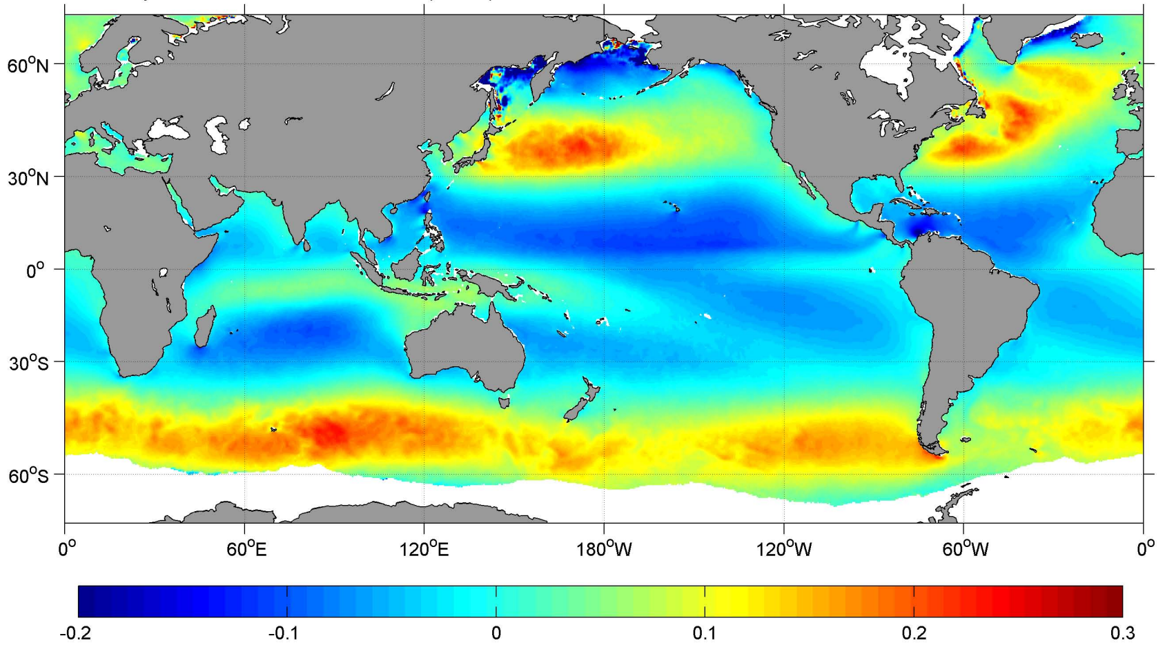
February SCOW Zonal Wind Stress ( \text{N m}^{-2} )
