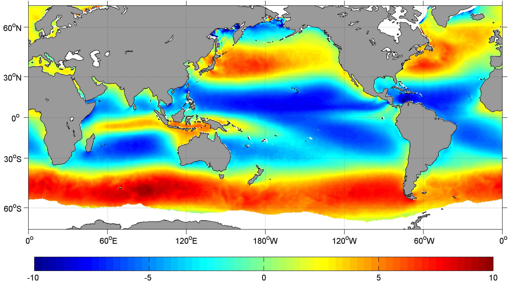
February SCOW Zonal Wind ( \text{m s}^{-1} )
