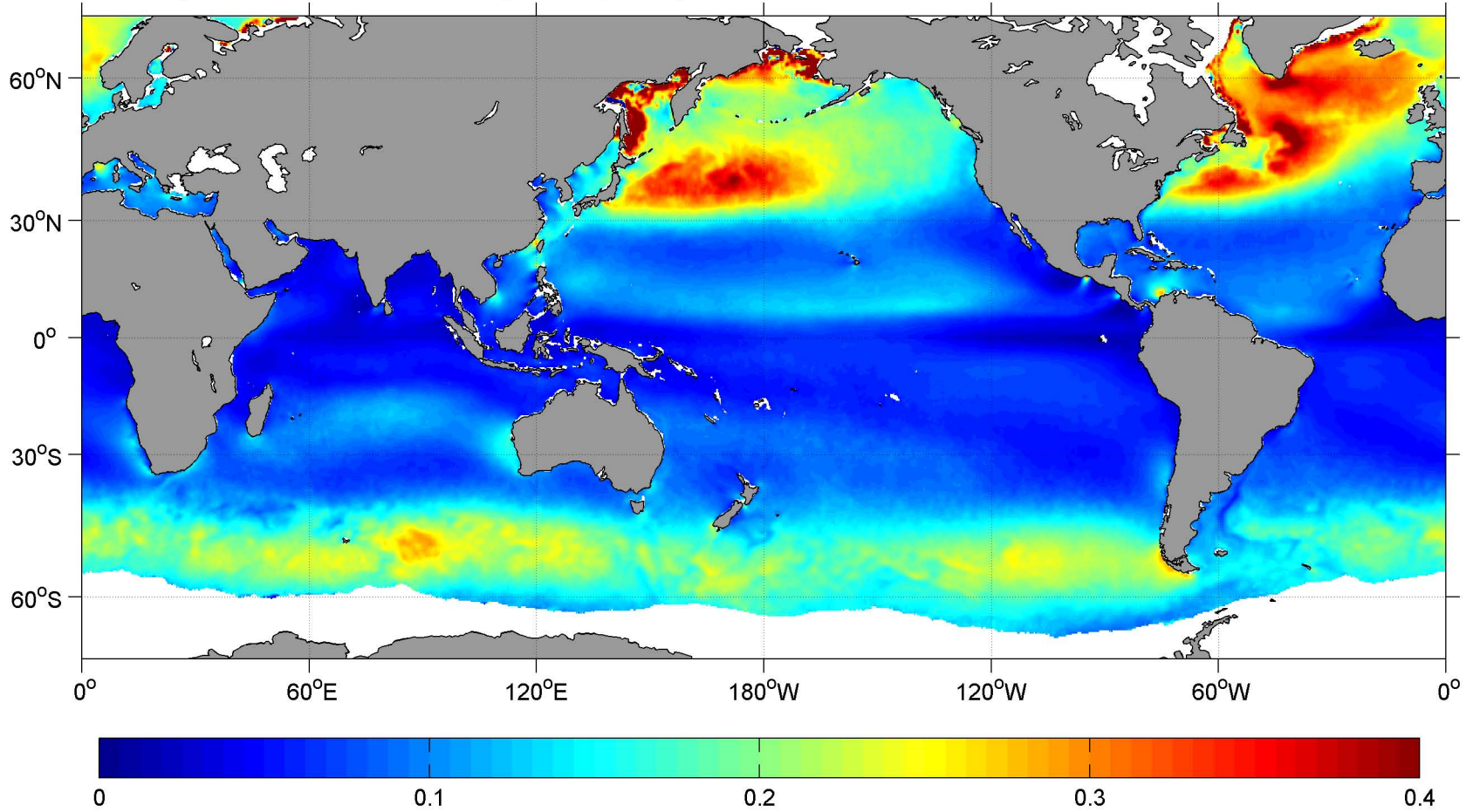
February SCOW Wind Stress Magnitude ( \text{N m}^{-2} )
