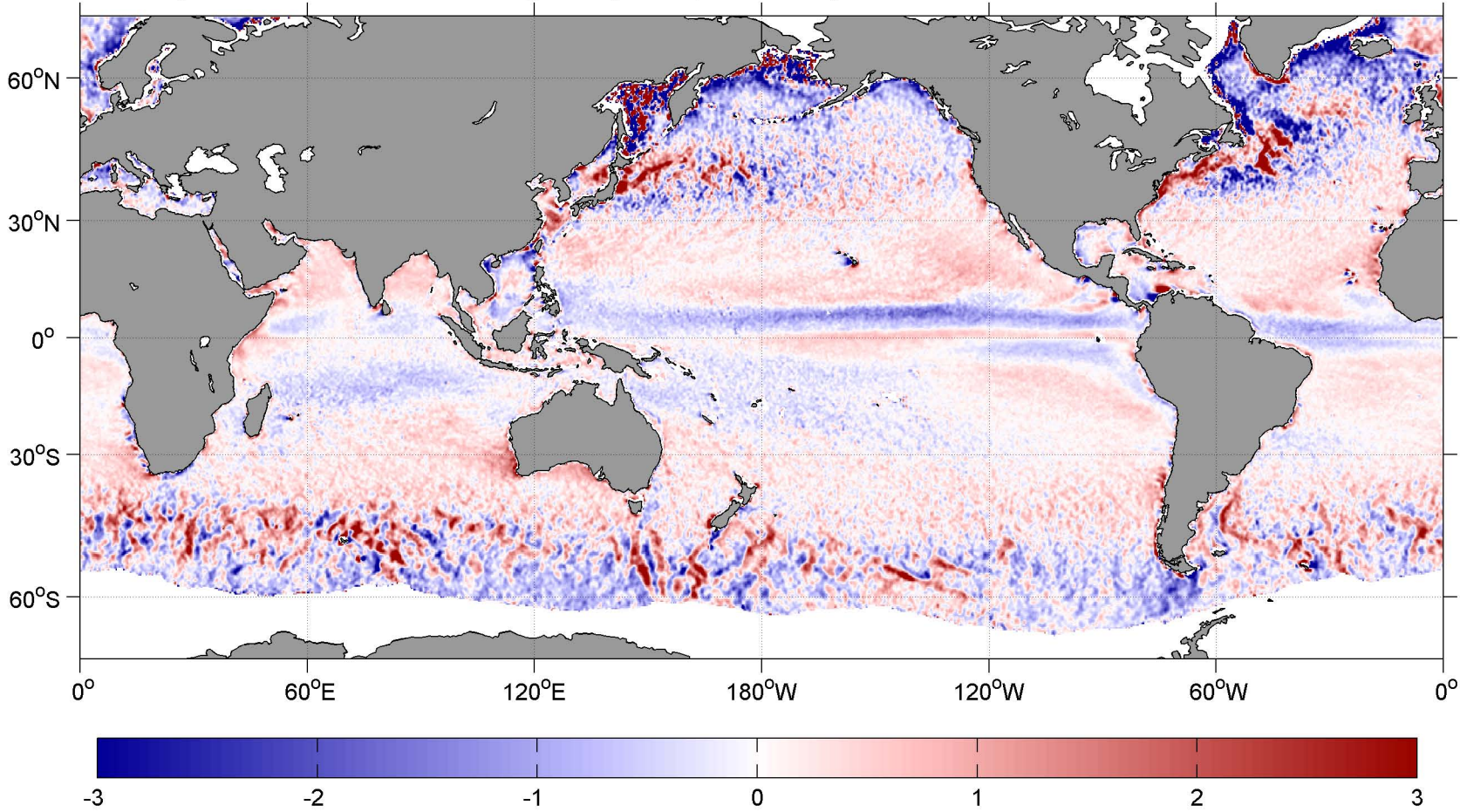
February SCOW Wind Stress Divergence ( \text{N m}^{-2} per 10^4 \text{ km}^2 )
