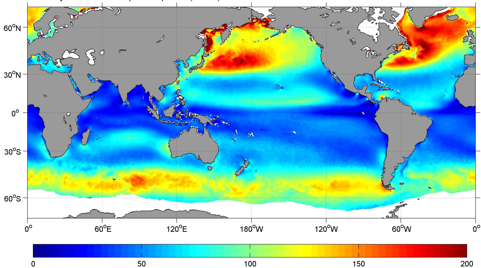
February SCOW Wind Speed Squared ( \text{m}^2 \text{s}^{-2} )
