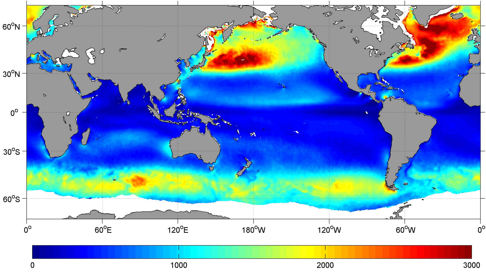
February SCOW Wind Speed Cubed ( \text{m}^3 \text{s}^{-3} )
