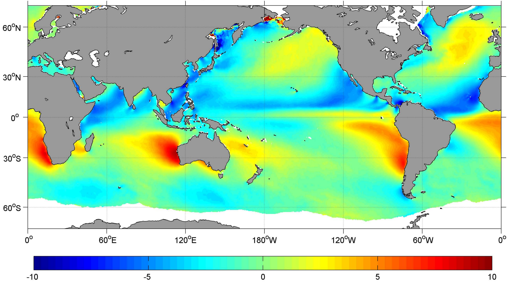
February SCOW Meridional Wind ( \text{m s}^{-1} )
