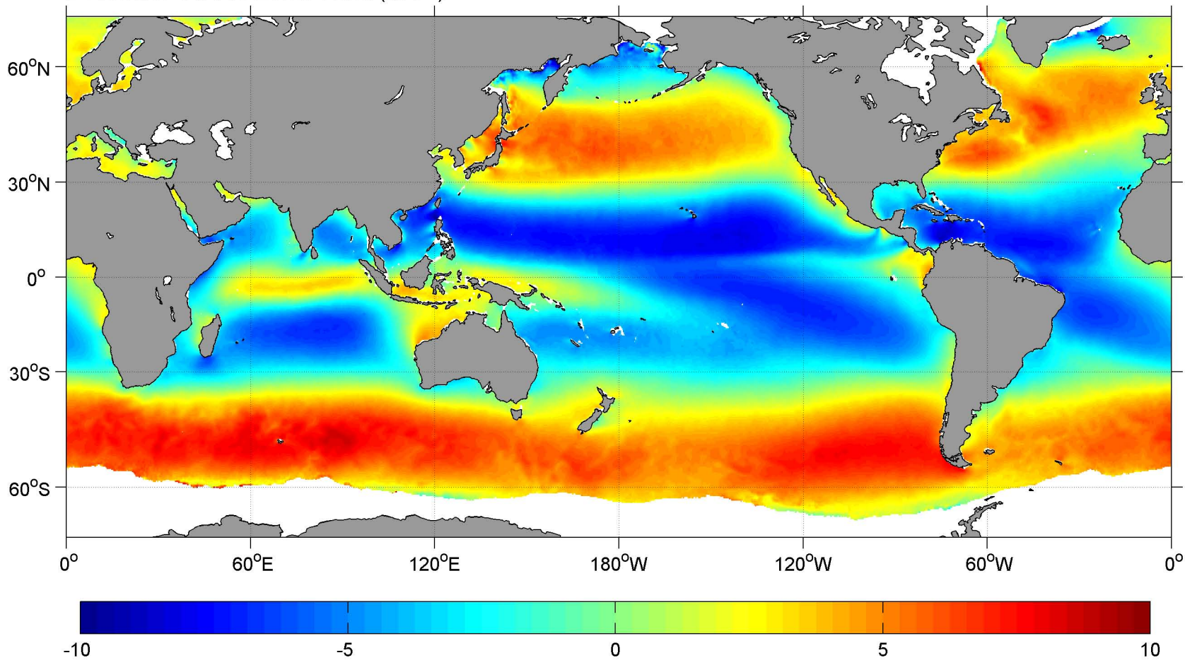
December SCOW Zonal Wind ( \text{m s}^{-1} )
