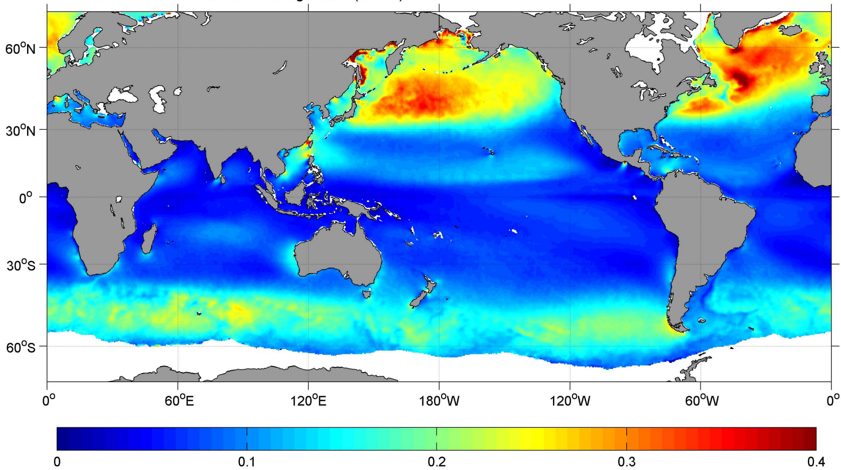
December SCOW Wind Stress Magnitude ( \text{N m}^{-2} )
