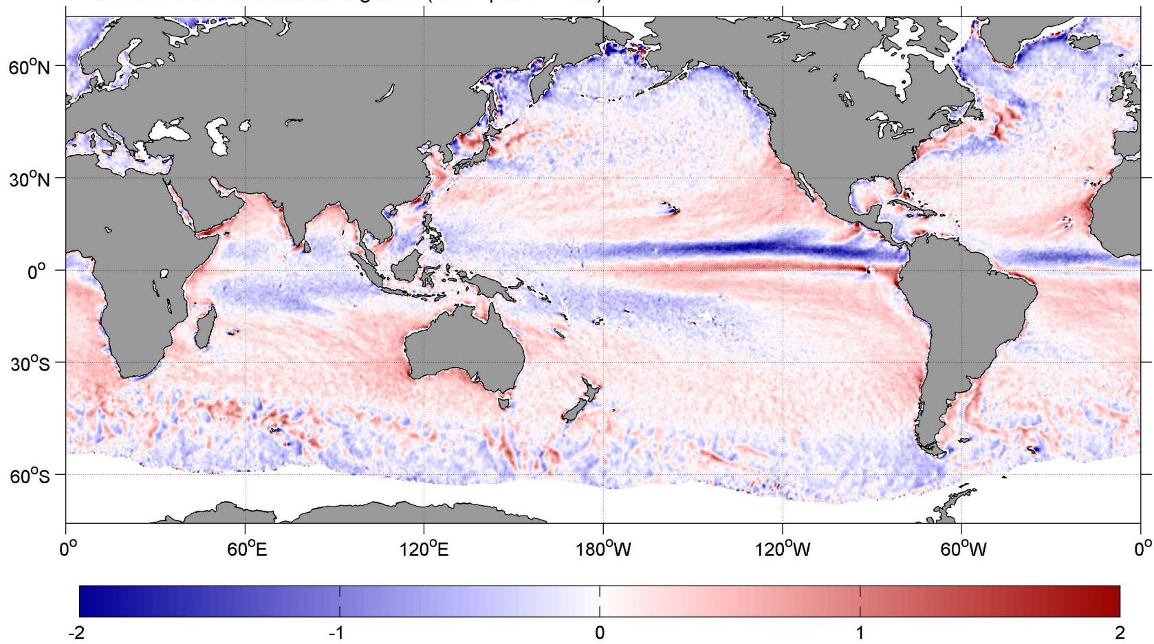
December SCOW Wind Divergence ( \text{m s}^{-1} per 10^2 \text{ km} )
