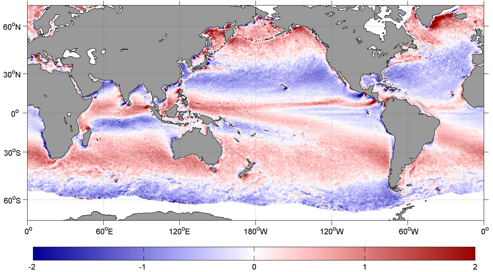
December SCOW Wind Curl ( \text{m s}^{-1} per 10^2 \text{ km} )
