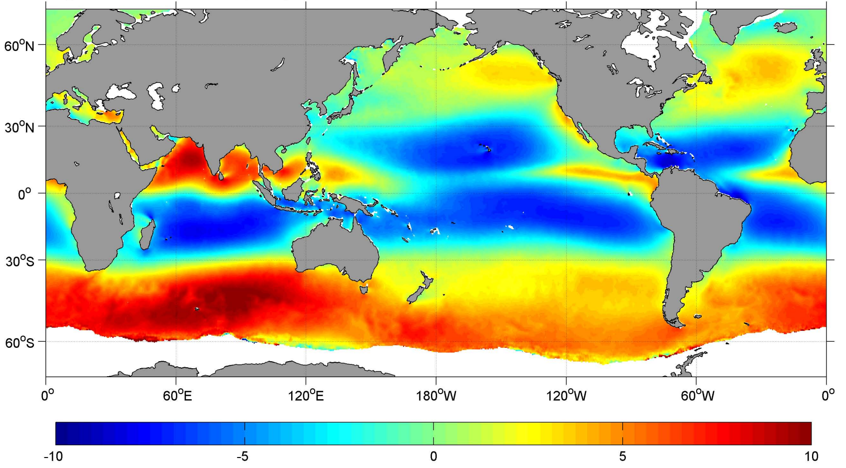
August SCOW Zonal Wind ( \text{m s}^{-1} )
