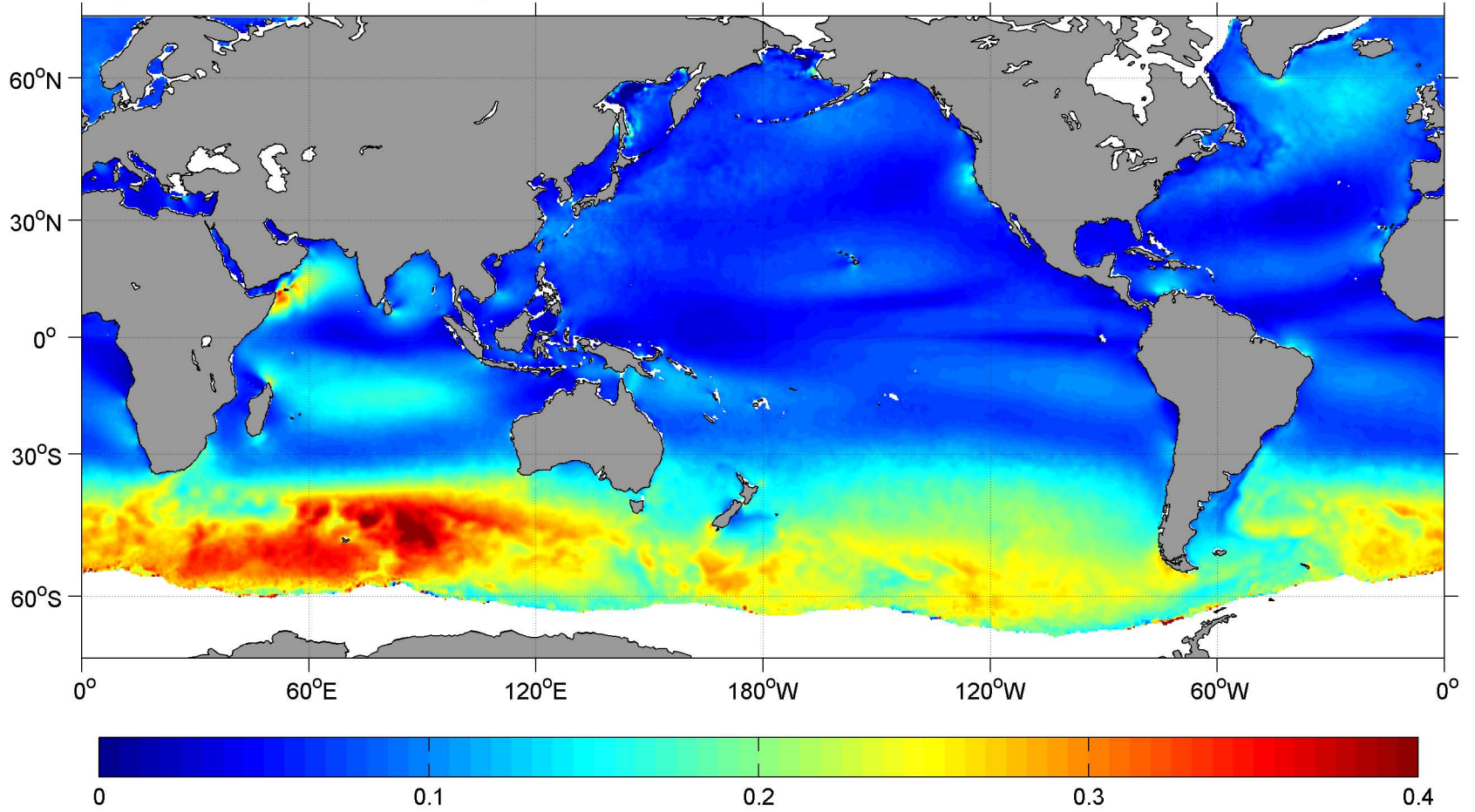
August SCOW Wind Stress Magnitude ( \text{N m}^{-2} )
