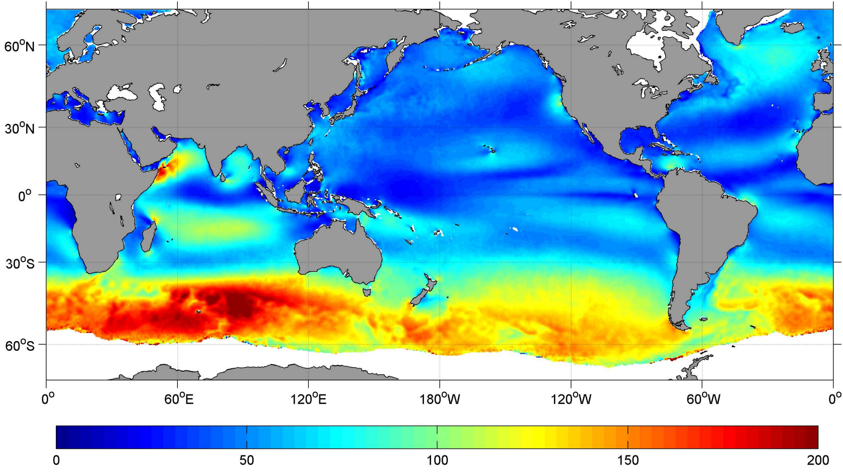
August SCOW Wind Speed Squared ( \text{m}^2 \text{s}^{-2} )
